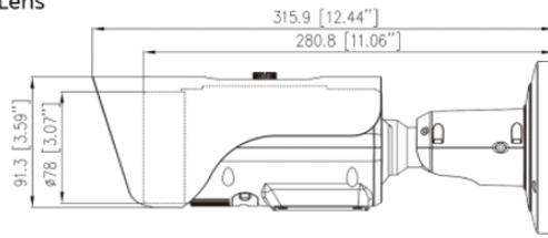
F25 / F35 / F50 mm Lens
